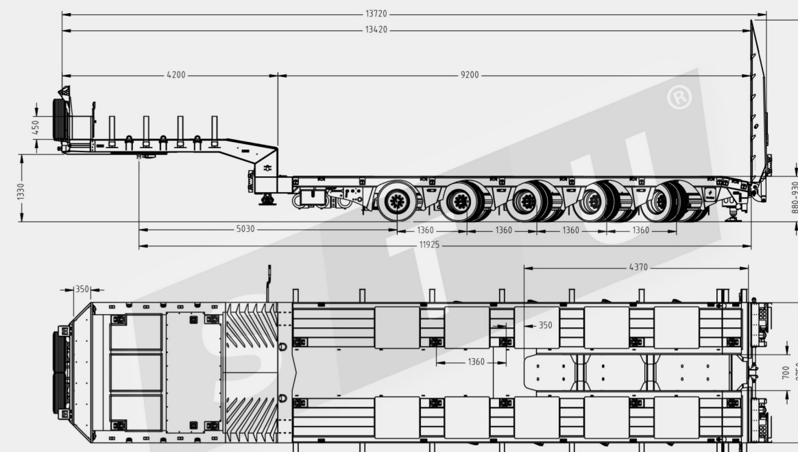
TECHNICAL DRAWING
