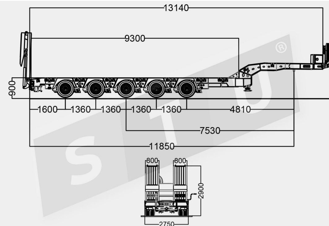
TECHNICAL DRAWING
