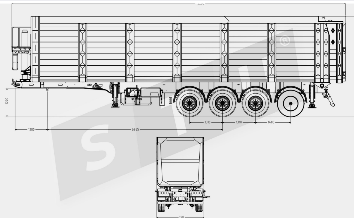
TECHNICAL DRAWING
