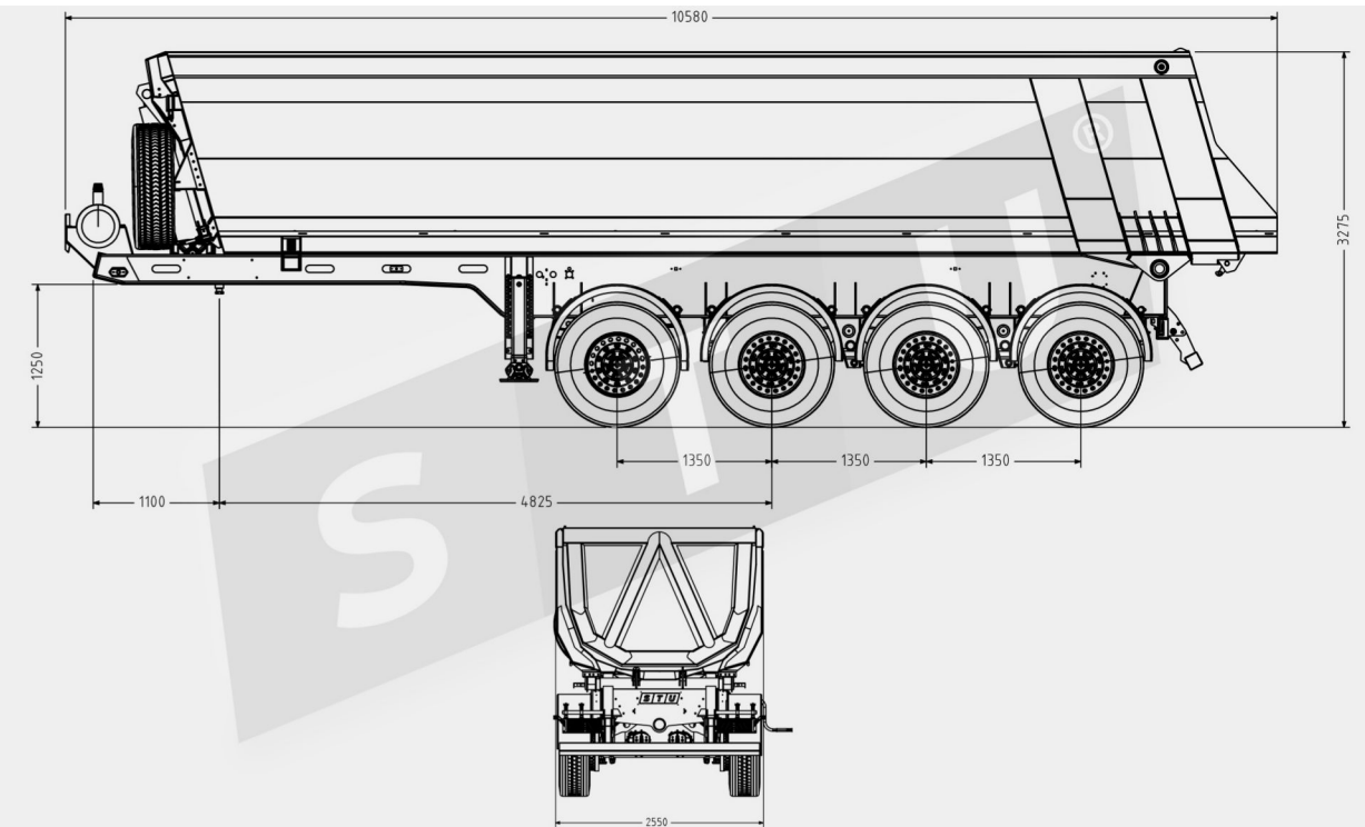
TECHNICAL DRAWING
