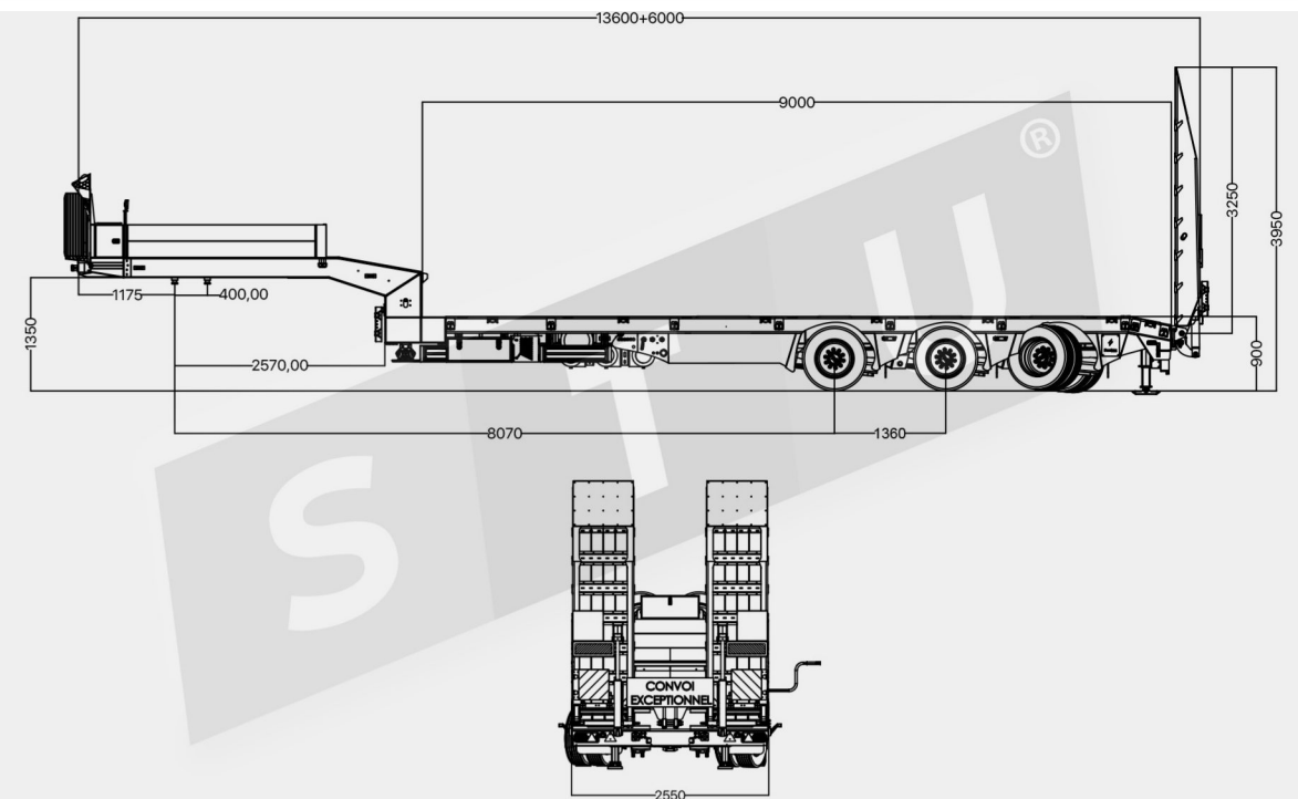
TECHNICAL DRAWING
