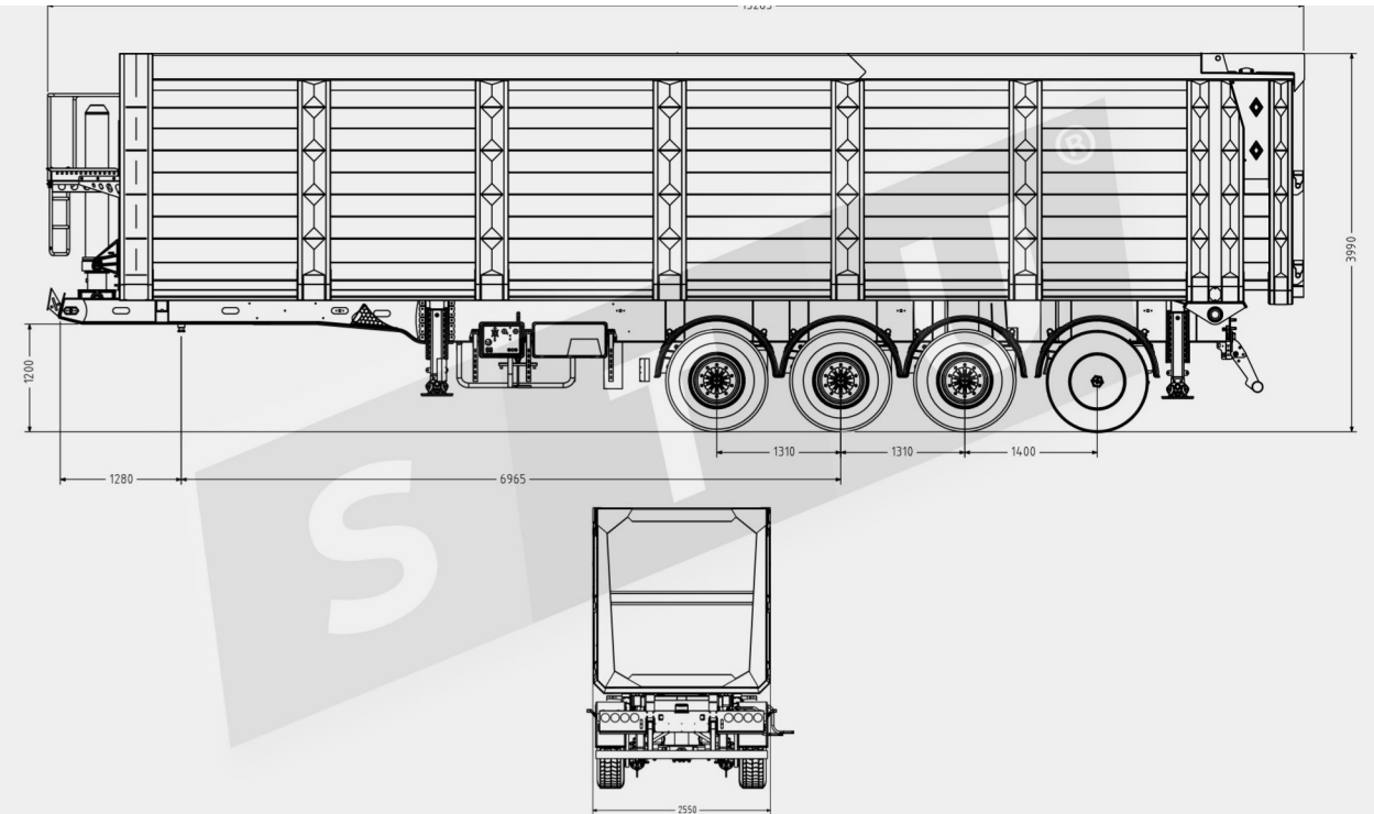
TECHNICAL DRAWING
